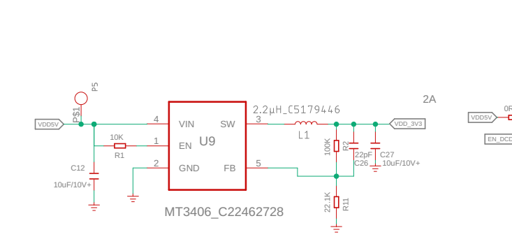
DC-DC:5V to 3V3
