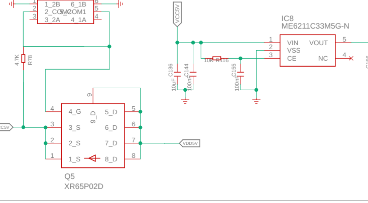
DC-DC:5V to 3V3
