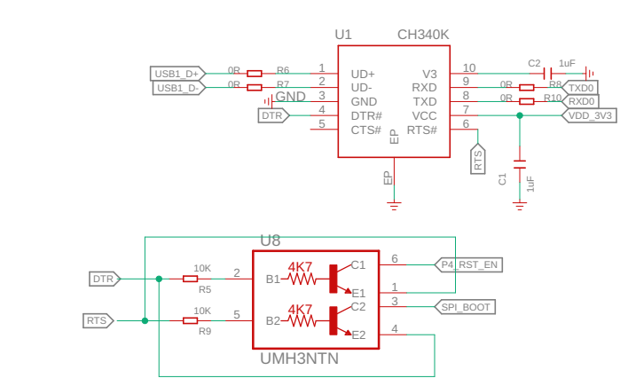
USB TO UART
