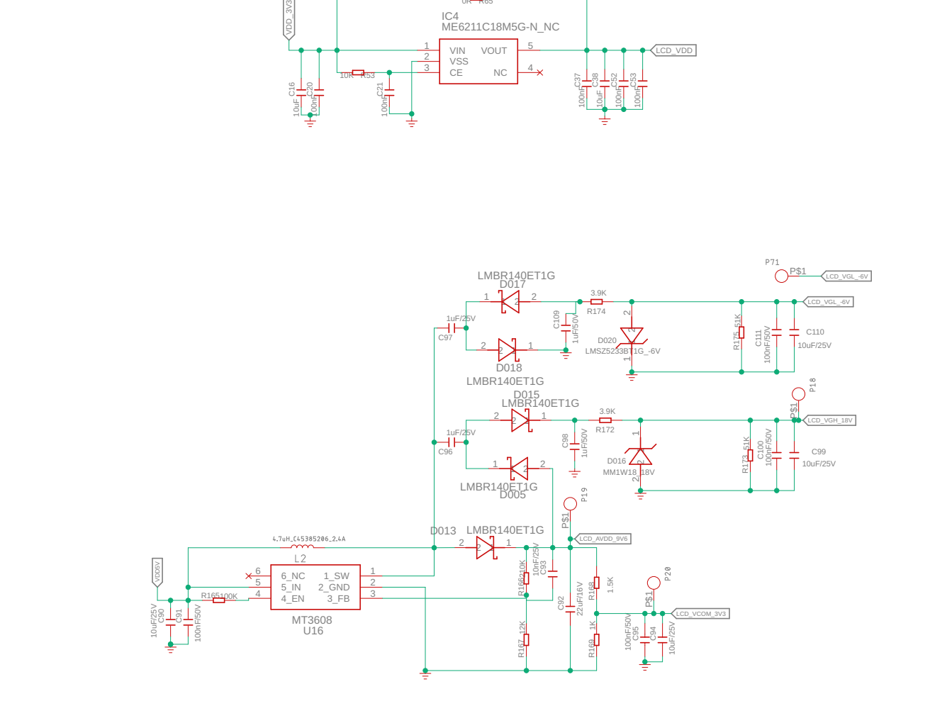
LCD_POWER
