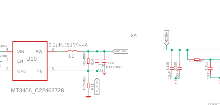
DC-DC:5V to 1V2
